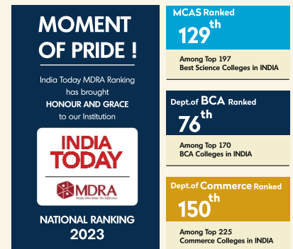
MDRA Ranking - 2023
